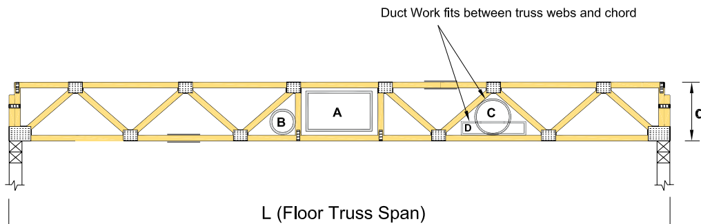
Figure 1. Typical 4 x 2 floor truss configuration with mechanical chase opening located near truss mid-span.
